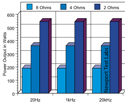
Power Output Test Result Graph: Single channel driven into 8-ohm, 4-ohm and 2-ohm non-inductive loads at 20Hz, 1kHz and 20kHz. [Audio Analogue Maestro Anniversary Integrated Amplifier]
