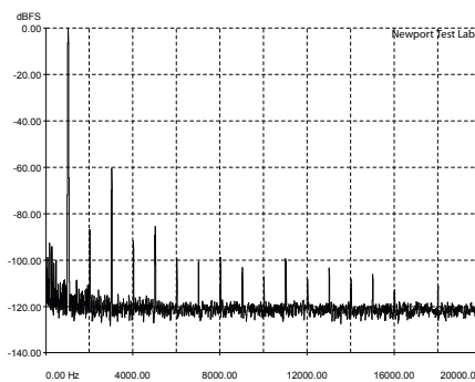
Graph 2: Total harmonic distortion (THD) at 1kHz at an output of 1-watt into a 4-ohm non-inductive load, referenced to 0dB. [Audio Analogue Maestro Integrated Amplifier]
