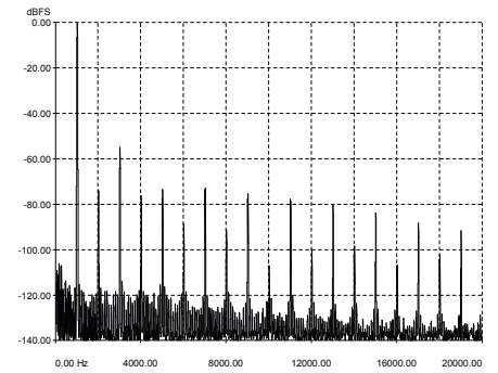
Graph 4: Total harmonic distortion (THD) at 1kHz at an output of 300-watts into a 4-ohm non-inductive load, referenced to 0dB. [Audio Analogue Maestro Integrated Amplifier]
