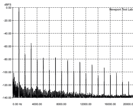
Graph 3: Total harmonic distortion (THD) at 1kHz at an output of 150-watts into an 8-ohm non-inductive load, referenced to 0dB. [Audio Analogue Maestro Integrated Amplifier]
