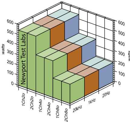
Power Output: Both channels driven into 8-ohm, 4-ohm and 2-ohm non-inductive loads at 20Hz, 1kHz and 20kHz. [Audio Analogue Maestro Anniversary Integrated Amplifier]
