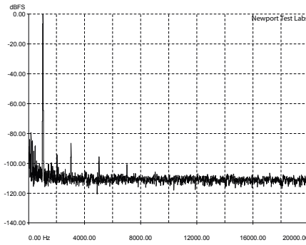
Graph 1: Total harmonic distortion (THD) at 1kHz at an output of 1-watt into an 8-ohm non-inductive load, referenced to 0dB. [Audio Analogue Maestro Integrated Amplifier]
