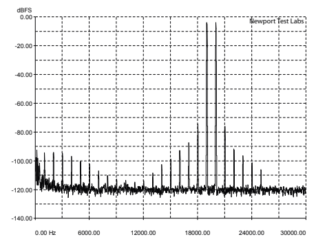
Graph 5: Intermodulation distortion (CCIF-IMD) using test signals at 19kHz and 20kHz, at an output of 1-watt into an 8-ohm non-inductive load, referenced to 0dB. [Audio Analogue Maestro Integrated Amplifier]
